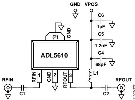
Figure 25. Basic Connections
