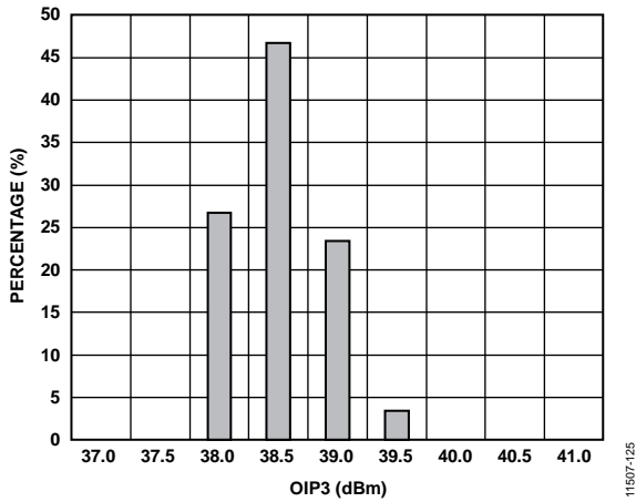
Figure 22. OIP3 Distribution at 900 MHz, P_{OUT} = 3 dBm per Tone
