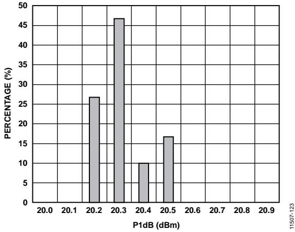
Figure 21. P1dB Distribution at 900 MHz
