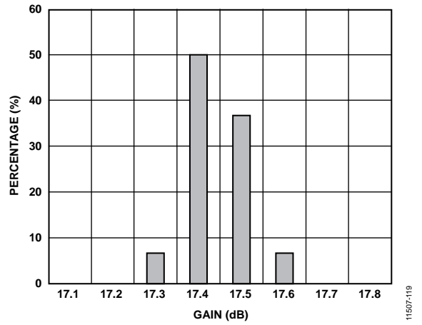
Figure 19. Gain Distribution at 2600 MHz
