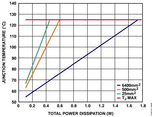
Figure 72. LFCSP, T_A = 50^\circ\text{C}
