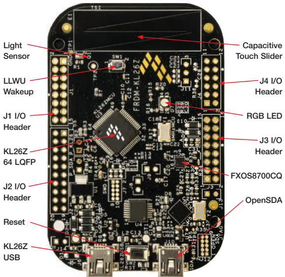
Figure 1: FRDM-KL26Z Callouts
