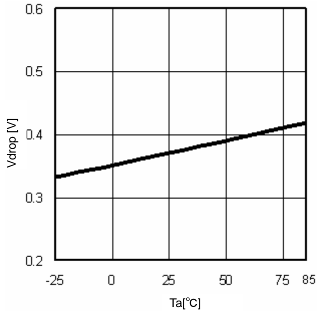
Fig.18 Minimum dropout Voltage1 (V cc =5V, I o =-0.5A)
