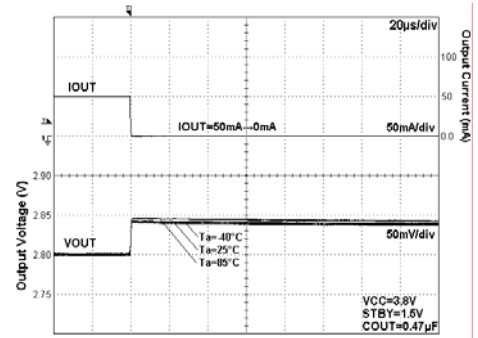
Fig 194. Load Response
