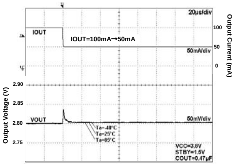
Fig 200. Load Response
