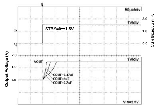
Fig 48. Start Up Time Iout=200mA
