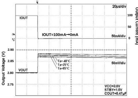
Fig 196. Load Response
