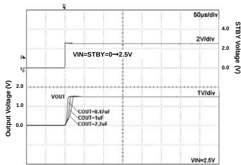
Fig 49. Start Up Time (VIN=STBY) Iout=0mA Iout=0mA
