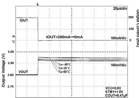
Fig 198. Load Response
