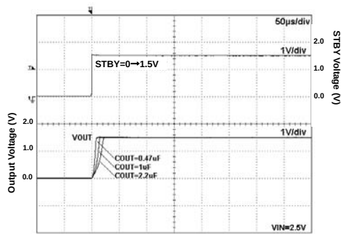
Fig 47. Start Up Time Iout=0mA
