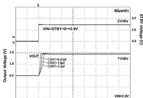
Fig 99. Start Up Time (VIN=STBY) Iout=0mA Iout=0mA
