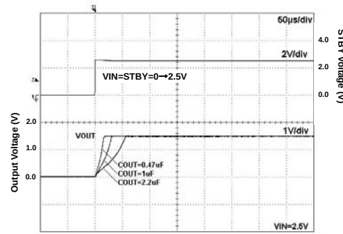
Fig 50. Start Up Time (VIN=STBY) Iout=200mA
