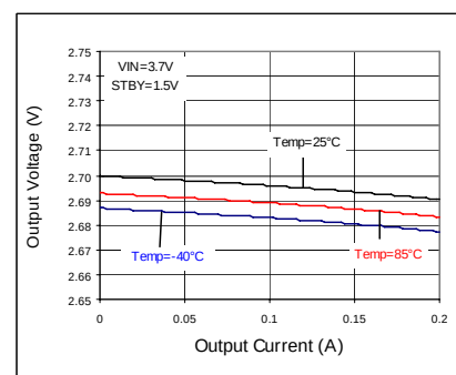
Fig 160. Load Regulation
