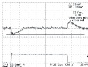
1.8V Transient Response
