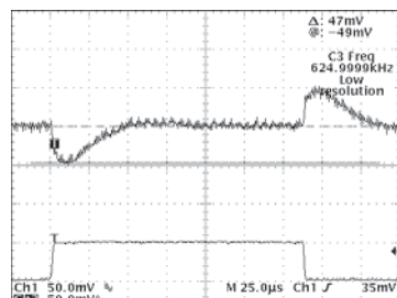
2.5V Transient Response
