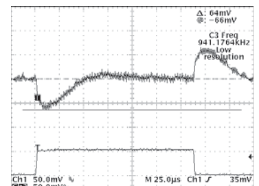
3.3V Transient Response
