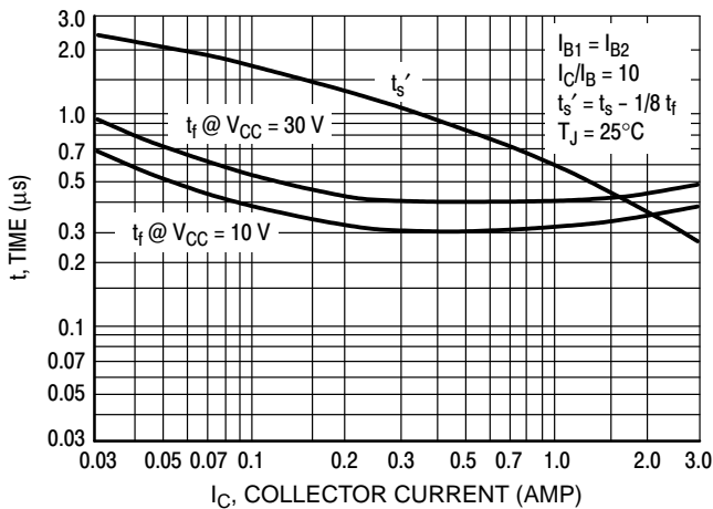
Figure 7. Turn-Off Time
