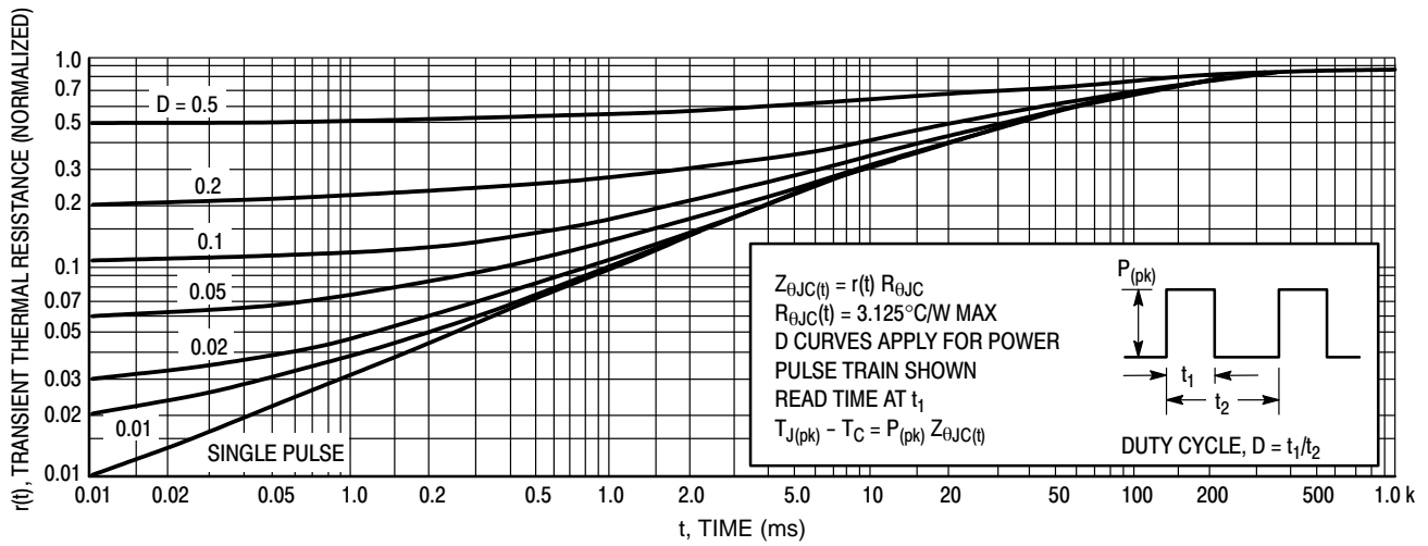
Figure 5. Thermal Response
