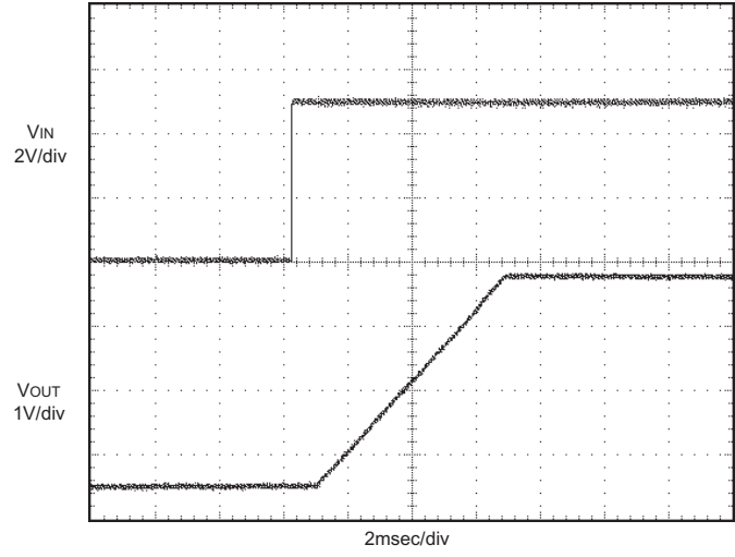
Start-Up from VIN (I OUT = 3.3V/10A, C IN /C OUT = 22μF)
