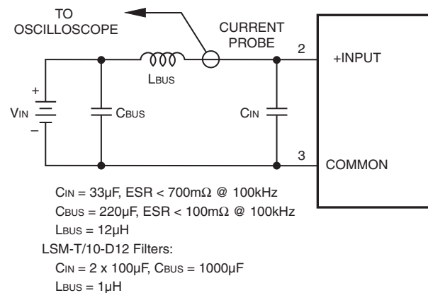
Figure 2. Measuring Input Ripple Current
