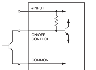
ON/OFF pin open: Logic High = DC/DC converter On ON/OFF pin <0.4V: Logic Low = DC/DC converter Off
