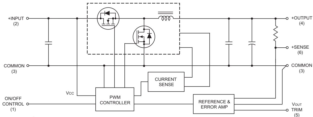
Figure 1. Simplified Schematic
