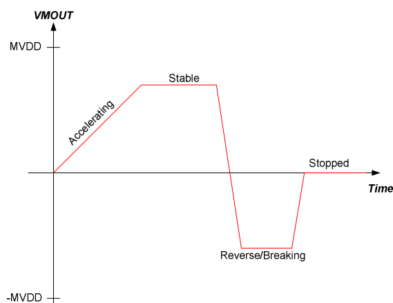
Figure 48 – ERM Drive Signal Example
