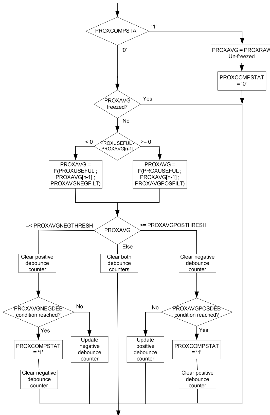
Figure 38 – ProxAvg Update
