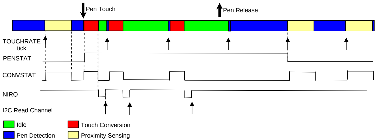
Figure 46 – Pen Trigger Mode (RegIrqMsk[6:2] = 00010 ; PROXSCANPERIOD = 001 ie 1/TOUCHRATE)
