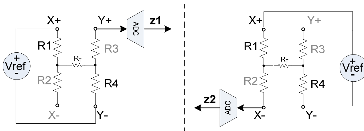
Figure 14 – Pressure Measurement
