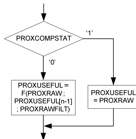
Figure 36 – PROXUSEFUL Update
