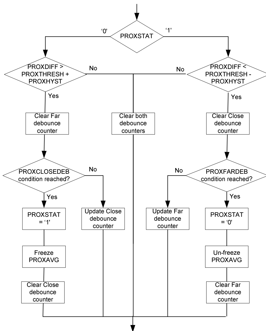
Figure 40 – PROXSTAT Update
