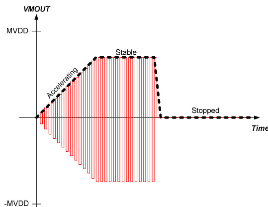
Figure 49 – LRA Drive Signal Example
