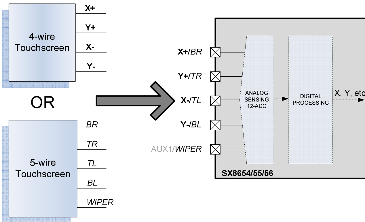
Figure 9 – Touchscreen Interface Overview
