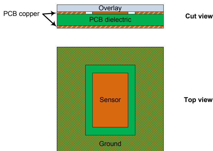
Figure 28 – Typical Capacitive Sensing Implementation
