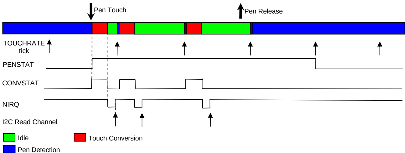
Figure 23 – Pen Trigger Mode ( \text{RegIrqMsk}[3:2] = 10 ; \text{PROXSCANPERIOD} = 0 )
