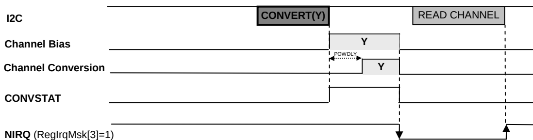
Figure 19 – Manual Mode – CONVERT Command (CHAN = Y; PROXSCANPERIOD = 0)
