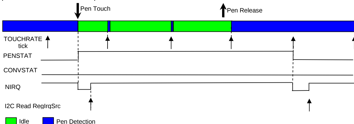
Figure 22 – Pen Detect Mode (RegIrqMsk[3:2] = 11 ; PROXSCANPERIOD = 0)
