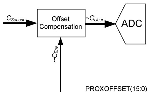
Figure 31 – Offset Compensation Block Diagram
