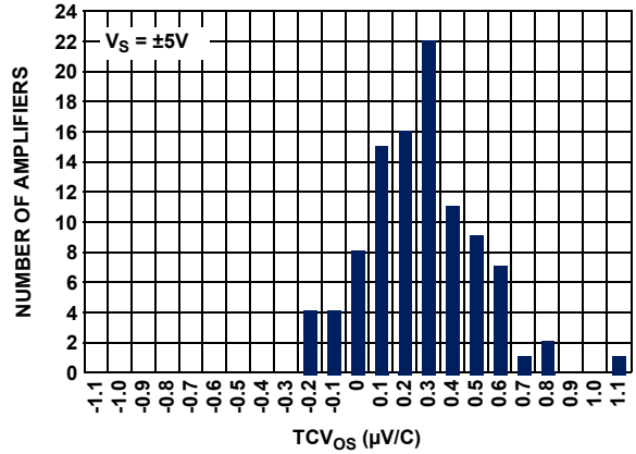
FIGURE 16. ISL28208 TDFN AND MSOP TCV 0S vs NUMBER OF AMPLIFIERS, V S = ±5V
