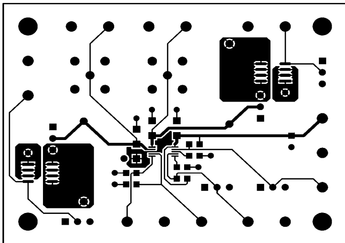
Top Copper
