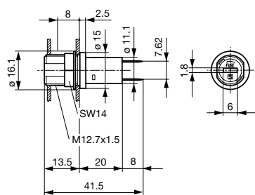
Variants 3101.0020 and 3101.0220
