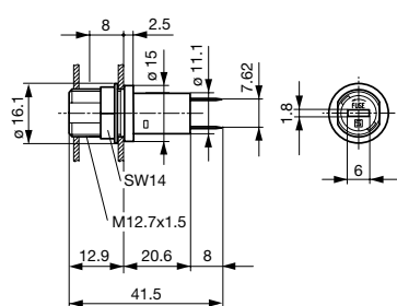
Variants 3101.0120 and 3101.0320
