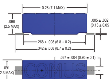
G-1 Model
