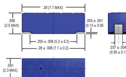
J-Lead Model
