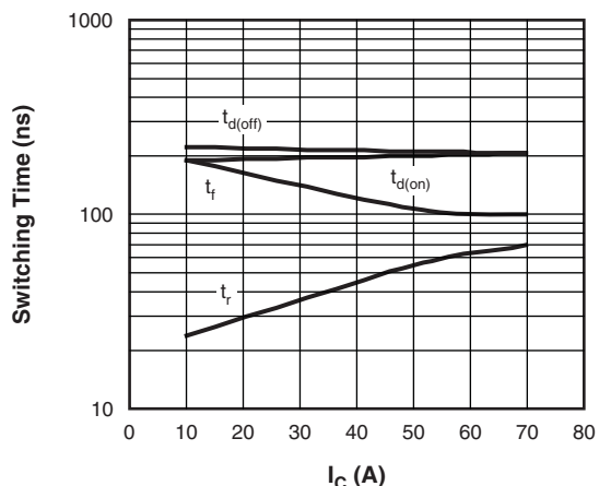
Fig. 10 - Typical IGBT Switching Time vs. I_C T_J = 125 °C, L = 500 μH, V_{CC} = 360 V, R_g = 5 Ω, V_{GE} = 15 V
