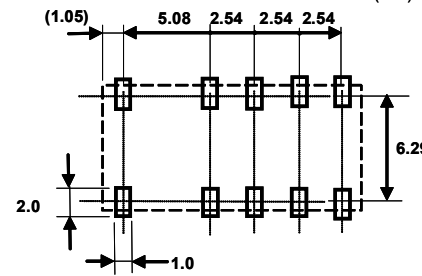
NOTE. General tolerance : \pm 0.1 (Top view)
