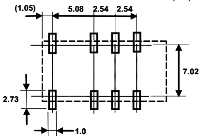
NOTE. General tolerance : \pm 0.1 (Top view)
