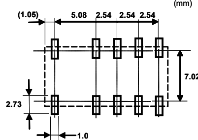
NOTE. General tolerance : \pm 0.1 (Top view)
