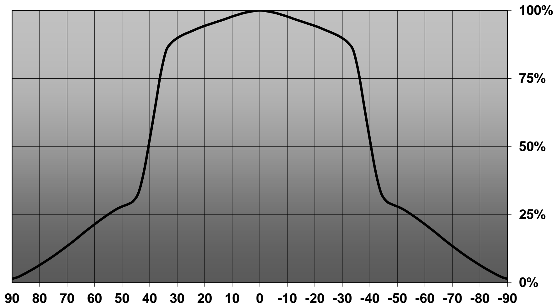
Relative intensity of C12469_LISA2-R-PIN (XB-D)
