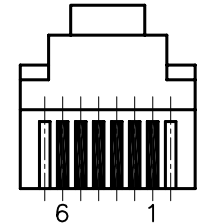
FRONT VIEW OF 8P6C TELEPHONE JACK
