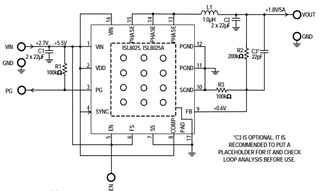
FIGURE 1. TYPICAL APPLICATION CIRCUIT CONFIGURATION (INTERNAL COMPENSATION OPTION)
