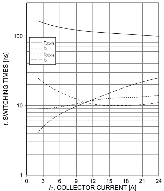
Figure 8. Typical switching times as a function of collector current (inductive load, T_{j}=150^{\circ}\text{C} , V_{CE}=400\text{V} , V_{GE}=15/0\text{V} , r_G=48\Omega , Dynamic test circuit in Figure E)
