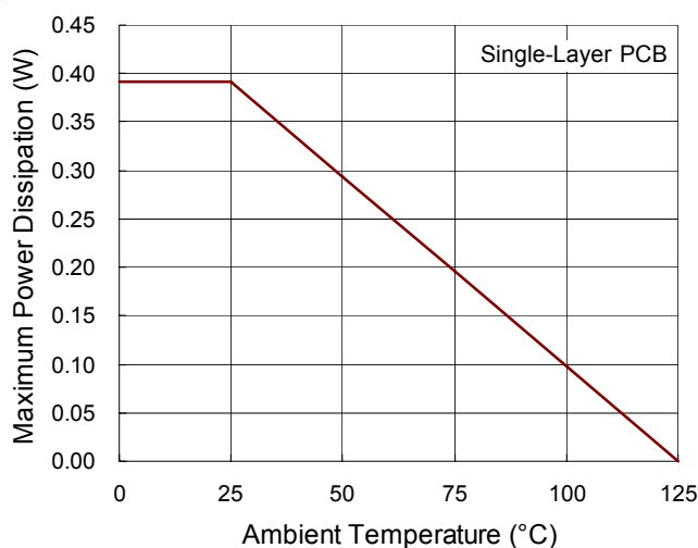
Figure 2. Derating Curve for RT8458 Package
