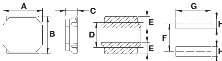
PCB Pattern
