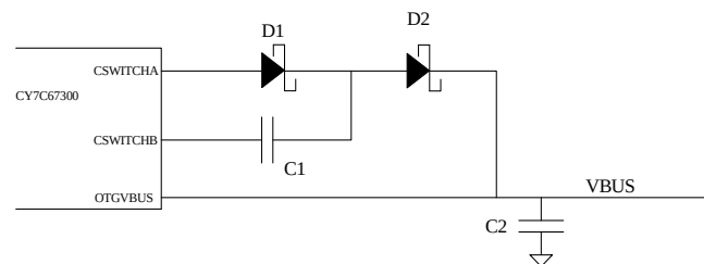
Figure 5. Charge Pump
