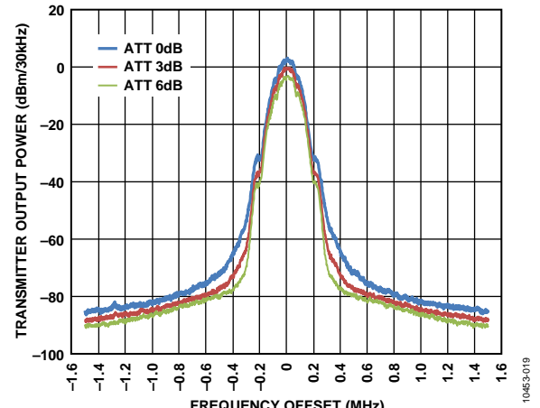
Figure 19. TX Spectrum vs. Frequency Offset from Carrier Frequency, f_{LO\_TX} = 800 MHz, GSM Downlink (Digital Attenuation Variations Shown), 3 MHz Range
