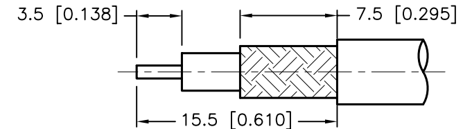
STRIPPING DIMENSION
