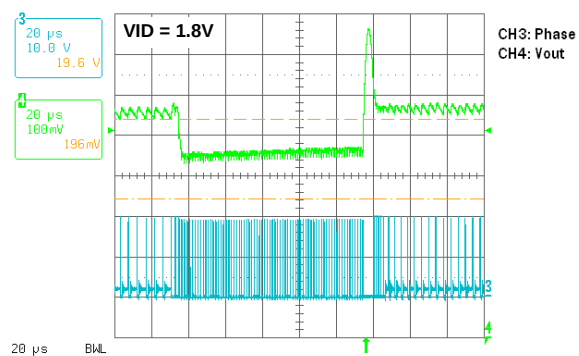
FIGURE 5. PS3 TO PS0, 1-35A TRANSIENT
