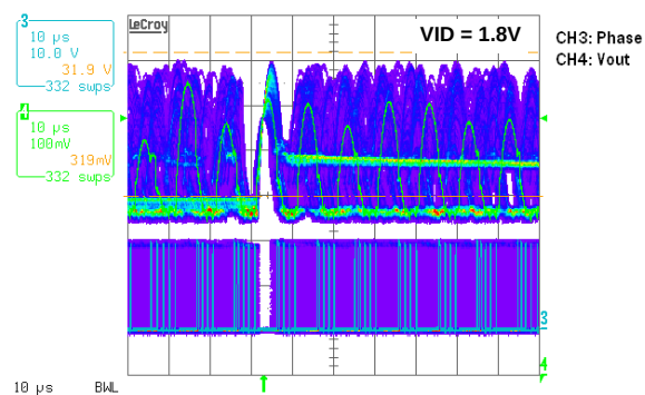
FIGURE 3. PS0, 1-35A HIGH REP LOAD TRANSIENT
