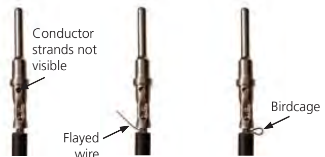
Unacceptable Crimps
