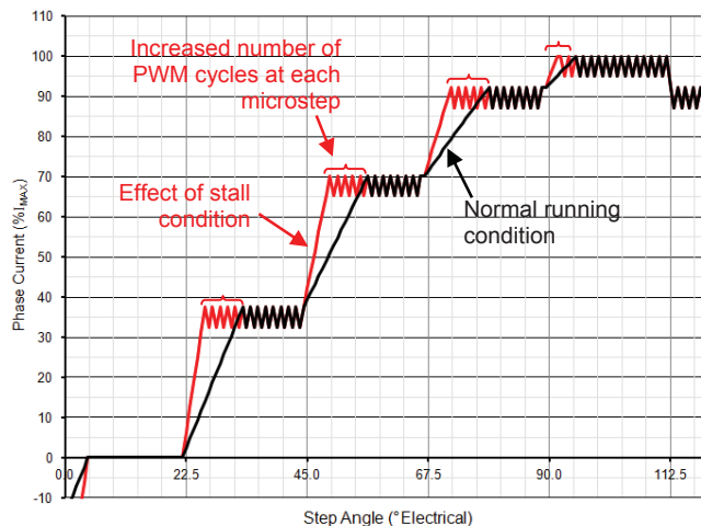
Figure 8. Effect of stall condition on current rise
