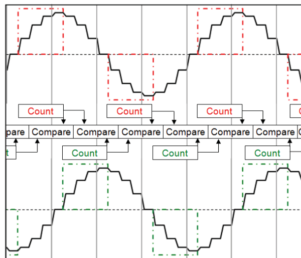
Figure 9. Stall detect by PWM count compare
