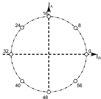
Figure 13. Half-step phase diagram using STEP input
