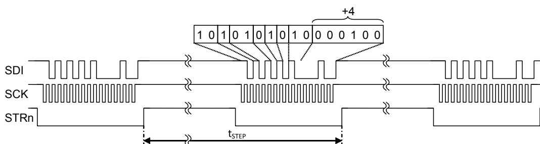
Figure 8. Serial interface sequence for quarter step in forward direction
