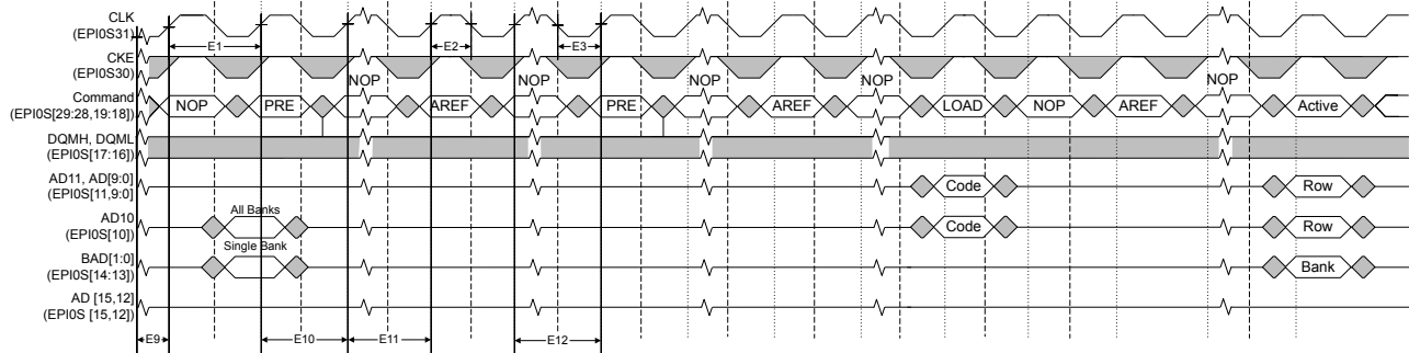
Figure 26-11. SDRAM Initialization and Load Mode Register Timing
