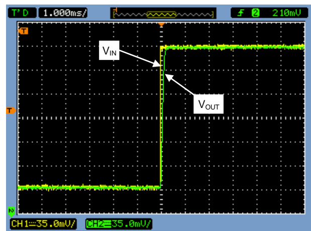
Figure 6: TS1003 Transient Response for R_{ISO} = 50\text{k}\Omega and C_{LOAD} = 500\text{pF} .
