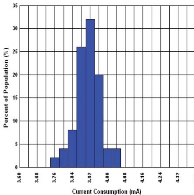
Figure 5.20 Current Consumption at +25°C
