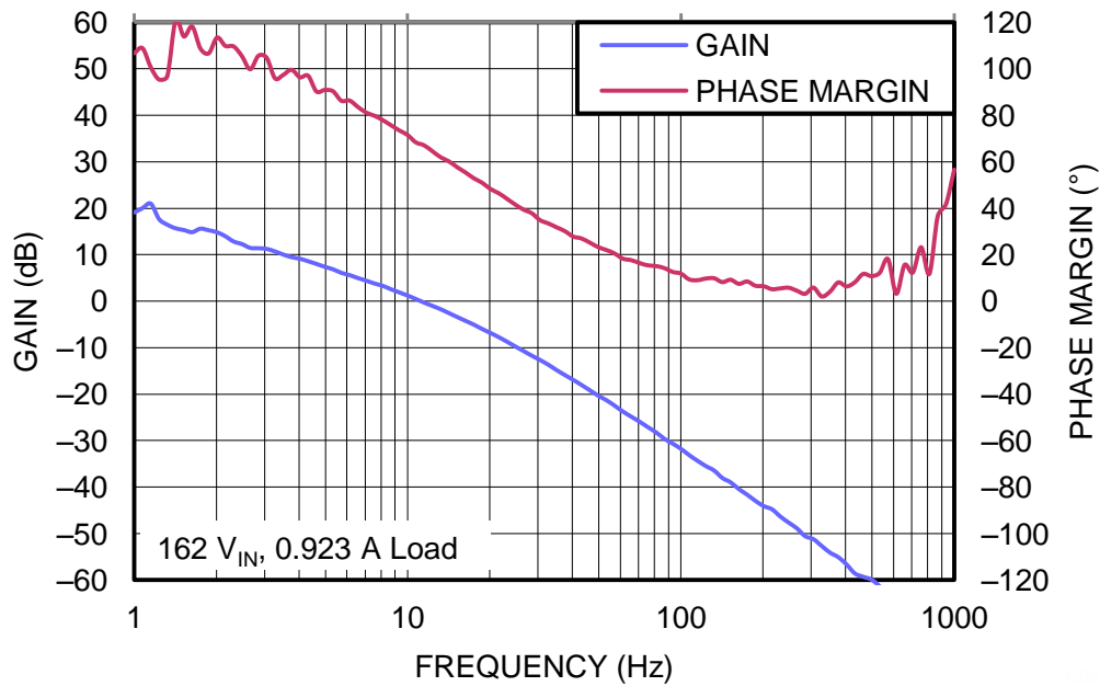
Figure 20. UCC28180EVM-573 Voltage Loop Response Gain and Phase, (311-V DC , full load, f CO = 10.7-Hz, phase margin = 68 degrees)
