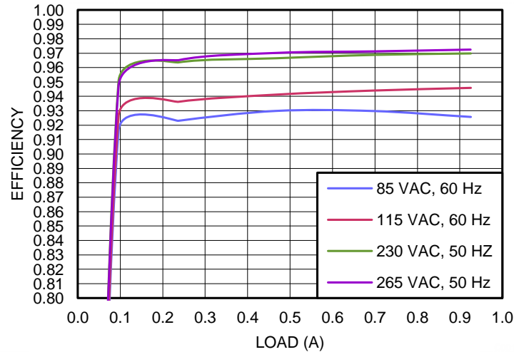
Figure 3. UCC28180EVM-573 Efficiency (as a function of line voltage and load current)
