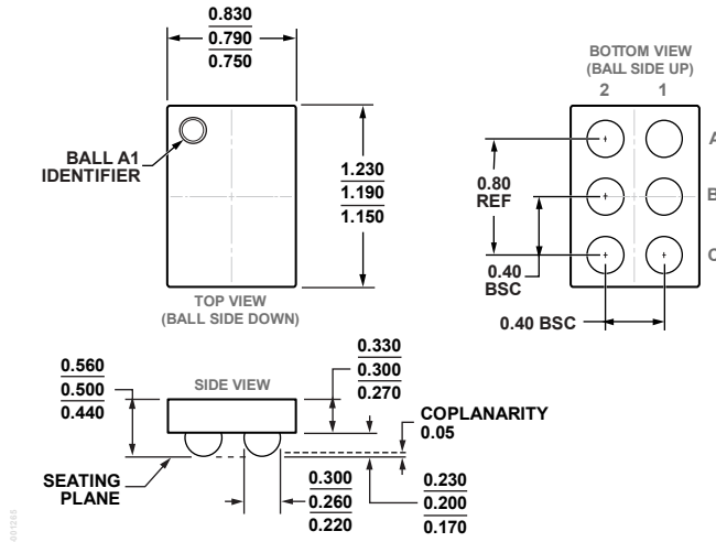
Figure 53. 6-Ball Wafer Level Chip Scale Package [WLCSP] (CB-6-14) Dimensions shown in millimeters
