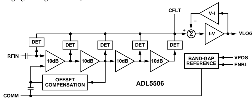
Figure 41. Block Schematic
