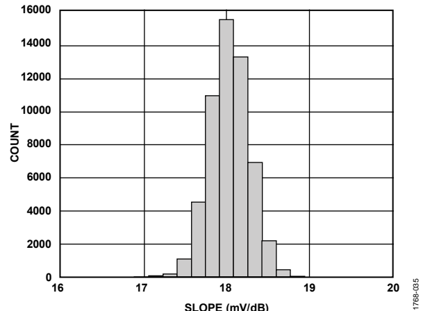
Figure 37. Distribution of Slope at 900 MHz, 25°C
