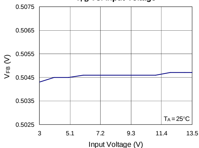
V FB vs. Input Voltage
