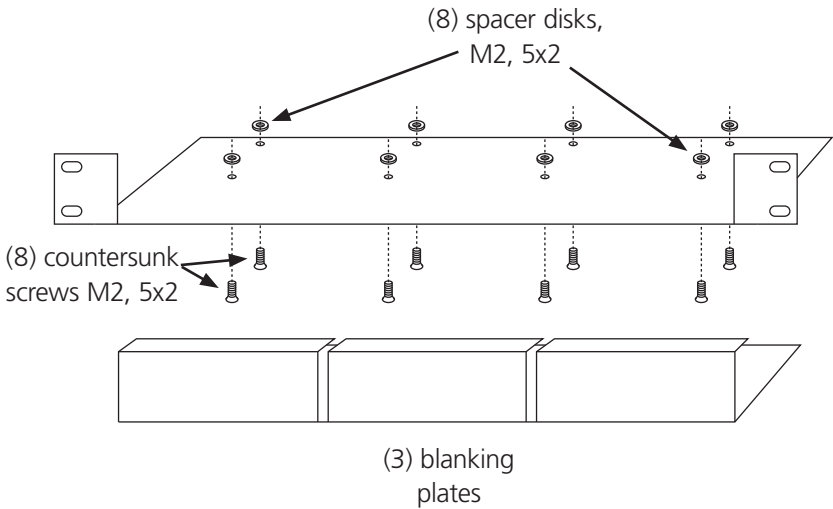
Figure 1. The Rackmount Kit's components.
