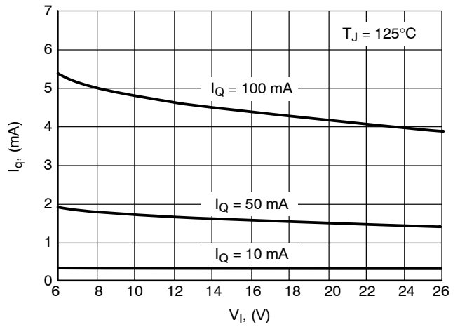
Figure 16. Quiescent Current I_q vs. Input Voltage V_I
