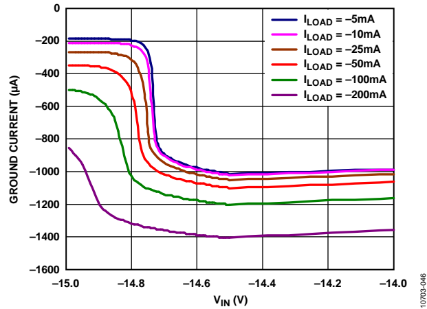
Figure 46. Ground Current vs. Input Voltage ( V_{IN} ) in Dropout, V_{OUT} = -15\text{ V}
