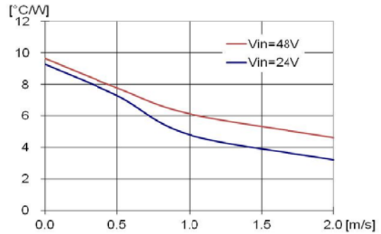
Figure 15. Thermal Resistance for the Open Frame Module; Airflow in the Transverse Direction from V_{out(-)} to V_{out(+)} ; V_{IN} = 24\text{V} or 48\text{V} , V_O=5.0\text{V} .
