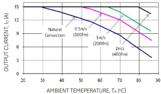
Figure 17. Output Current Derating for the Module with Heatplate; Airflow in the Transverse Direction from V_{out(-)} to V_{out(+)} ; V_{IN} = 48\text{V} , V_O=5.0\text{V} .
