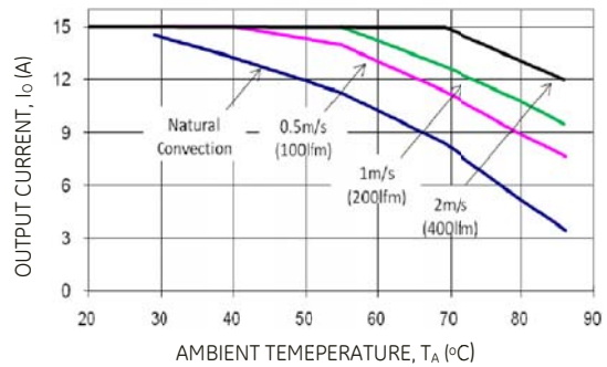
Figure 16. Output Current Derating for the Open Frame Module; Airflow in the Transverse Direction from V_{out(-)} to V_{out(+)} ; V_{IN} = 48\text{V} , V_O=5.0\text{V} .
