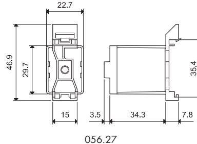
Top flange mount adaptor for 56.34
