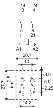
56.42-0300 Copper side view
