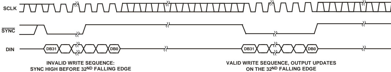
Figure 50. \overline{\text{SYNC}} Interrupt Facility
