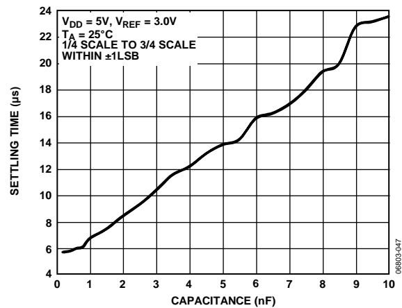
Figure 36. Settling Time vs. Capacitive Load
