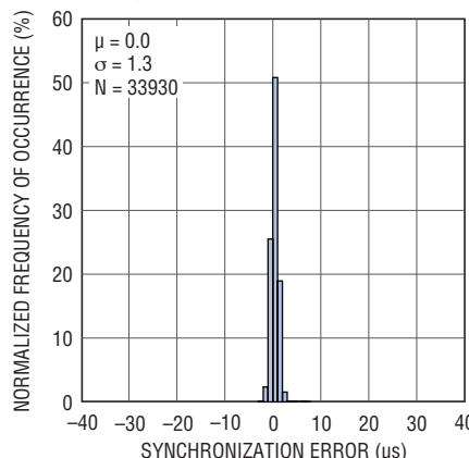
TIMEn Synchronization Error 1 Packet/s Publishing Rate, 3 Hops, 8°C/Min
