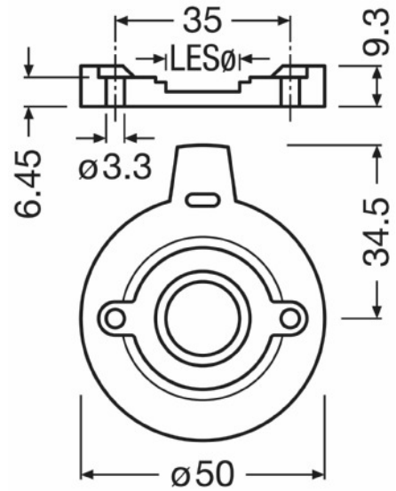
Product line drawing LEP -800-827-C-AC | LEP -800-830-C-AC | LEP -800-840-C-AC
