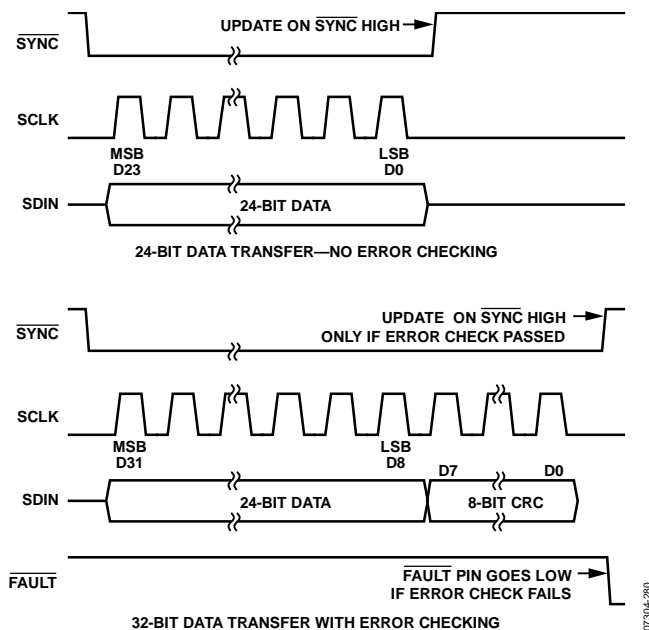
Figure 77. PEC Timing
