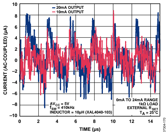
Figure 51. Output Current vs. Time with DC-to-DC Converter (See Figure 78)
