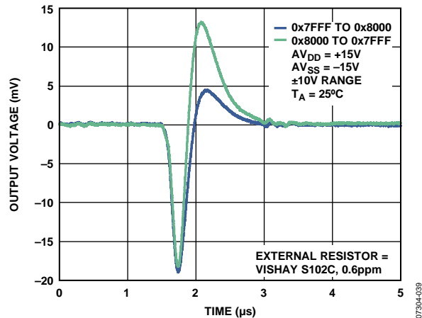
Figure 25. Digital-to-Analog Glitch
