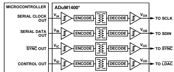
Figure 86. Isolated Interface
