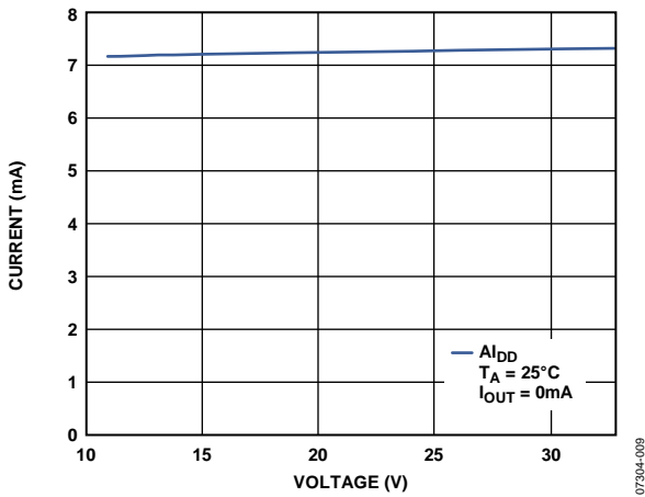
Figure 67. I_{DD} vs. AV_{DD}
