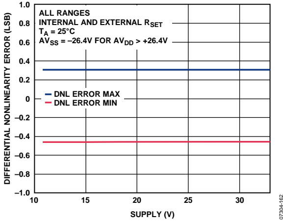
Figure 43. Differential Nonlinearity Error vs. AV_{DD}
