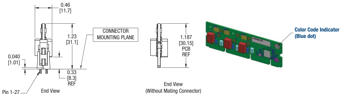
Figure 6. VR110B080CU-1C (80A, 1U)
