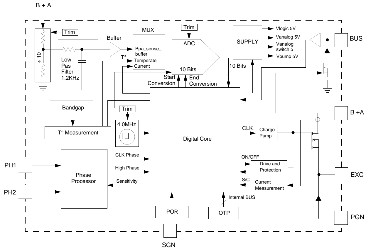
Figure 3. 80310 Simplified Internal Block Diagram
