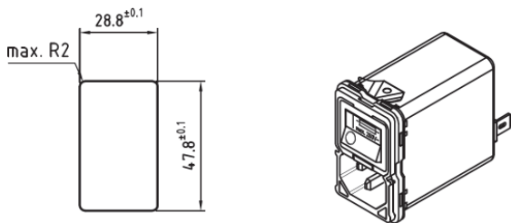
Panel cutout:
