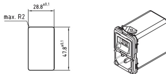
Panel cutout:
