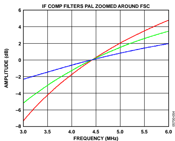
Figure 35. PAL IF Filter Compensation
