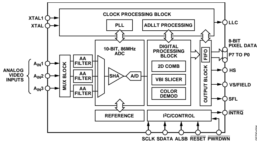
Figure 4. 64-Lead LQFP Functional Block Diagram
