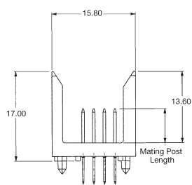
Solder Leads
