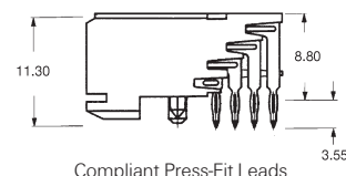
Compliant Press-Fit Leads
