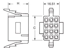
Socket Housing
