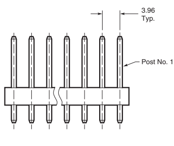
Flat Headers - Straight
