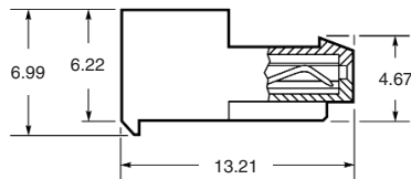
Without polarizing tabs
