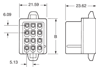
Pin Housing
