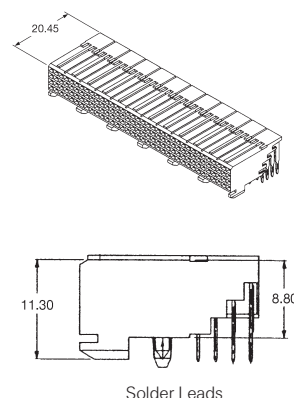
Solder Leads
