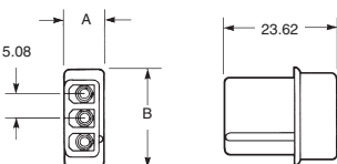
Pin Housing
