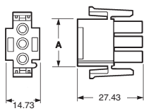
Plug
