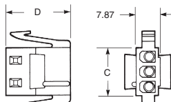
Socket Housing
