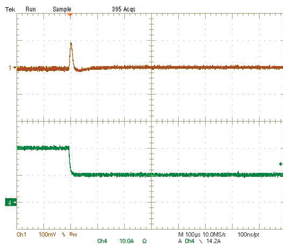
Step Load Transient Response (Vin=12V, Vout=2.5V, Cload=188µF, Iout=20A to 10A) Trace 1=Vout, 100 mV/div(AC), Trace 4=Iout, 10A/div.
