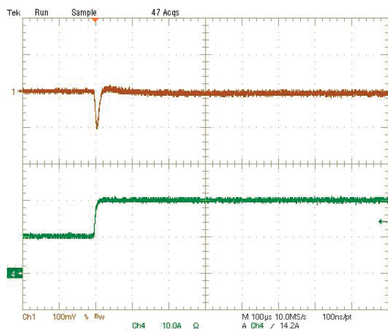
Step Load Transient Response (Vin=12V, Vout=2.5V, Cload=188µF, Iout=10A to 20A) Trace 1=Vout, 100 mV/div(AC), Trace 4=Iout, 10A/div.
