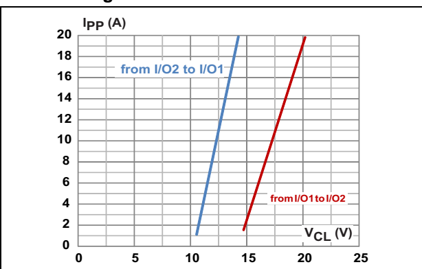
Figure 14. TLP measurement
