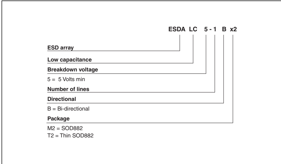
Figure 26. Ordering information scheme
