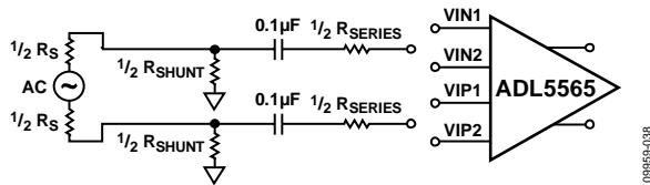
Figure 36. Gain Adjustment Using a Series Resistor
